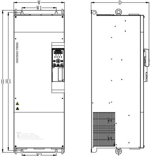
图 8-4 H150-4T37GB~H150-4T200G H150-4T315G~H150-4T450G 安装尺寸示意图
